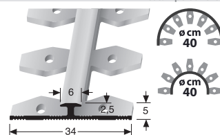
PF 363 EB \varnothing 2,5 mm
